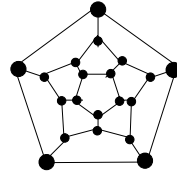
Dodecahedron
