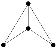
Tetrahedron
