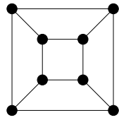
Hexahedron (Cube)
